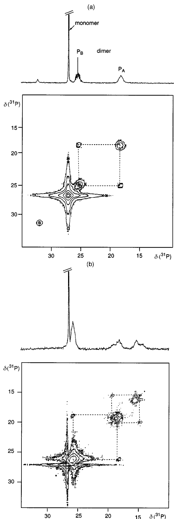
Fig. 4 Phase-sensitive ^{31}\text{P}\{^1\text{H}\} COSY spectra of the solution of \{[\text{Au}(\text{d2pype})_2]\text{Cl}\}_n in \text{CH}_3\text{OH} –30% \text{CH}_3\text{OD} at (a) 273 K and (b) 213 K with the ^{31}\text{P}\{^1\text{H}\} spectra shown as projections. The connectivities in (a) are between the \text{P}_\text{A} and \text{P}_\text{B} multiplets of the dimer, whereas in (b) although the connectivities between the \text{P}_\text{A} and \text{P}_\text{B} and \text{P}_\text{B} and \text{P}_\text{C} multiplets are consistent with both trimeric and tetrameric species, the relative intensities of the peaks are consistent with the tetrameric species (see text).
