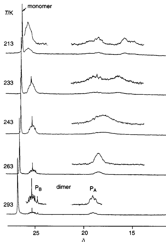
Fig. 3 161.9 MHz ^{31}\text{P}\{^1\text{H}\} NMR spectra of [\{\text{Au}(\text{d2pype})_2\}\text{Cl}]_n in \text{CH}_3\text{OH}-30\% \text{CH}_3\text{OD} at 293, 263, 243 and 233 and 213 K. The resonances at 293 K are assigned to the monomeric and dimeric species [\{\text{Au}(\text{d2pype})_2\}]^+ . A minor peak (not shown) representing ca. 4% of the total Au-P species is also observed at \delta 31.4. On cooling this peak broadened and disappeared below 253 K. Although unassigned its chemical shift is similar to [(\text{AuCl})_2(\text{d2pype})] (Fig. 1).
