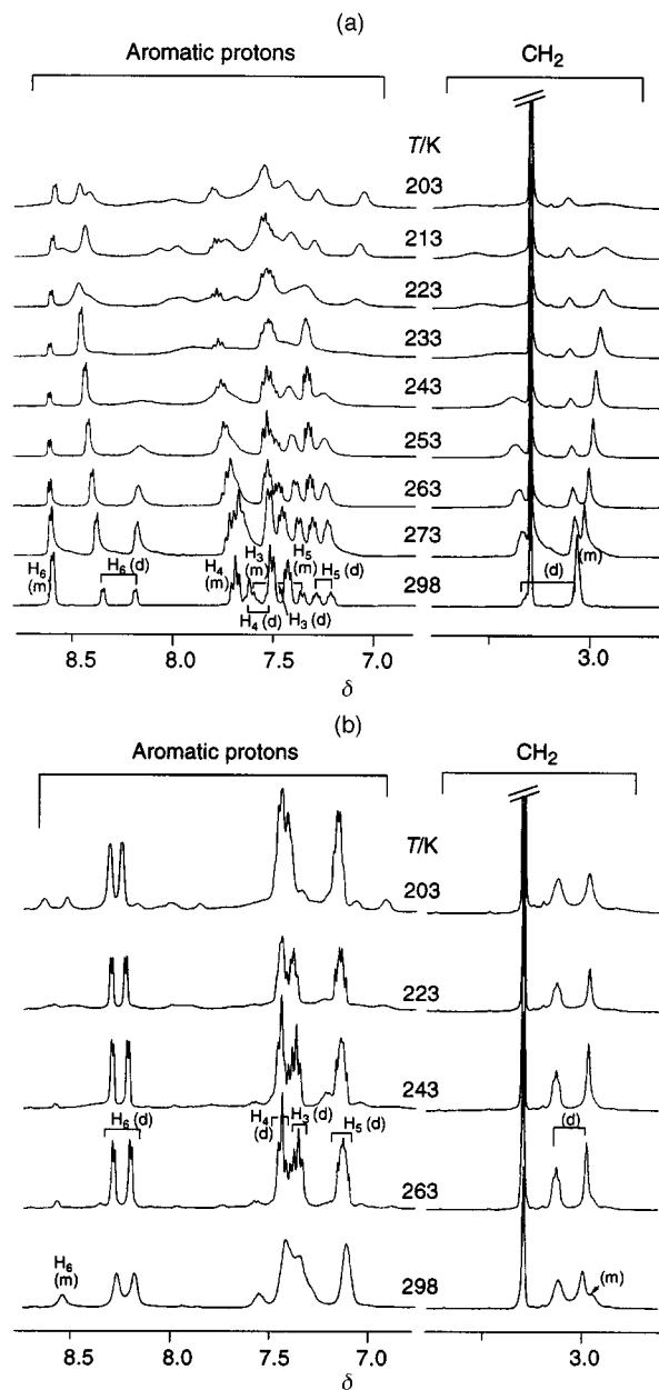
Fig. 5 ^1\text{H} spectra of (a) \{[\text{Au}(\text{d2pype})_2]\text{Cl}\}_n and (b) \{[\text{Ag}(\text{d2pype})_2]\text{NO}_3\}_n in \text{CD}_3\text{OD} at various temperatures, showing assignments for pyridyl and \text{P}(\text{CH}_2)_2\text{P} protons in monomeric (m) and dimeric (d) species. For the \text{Ag}(\text{I}) system the additional peaks visible below 263 K are assignable to the trimeric cluster \{[\text{Ag}(\text{d2pype})_2]\text{NO}_3\}_3 and the three species are in slow exchange on the NMR time scale.
